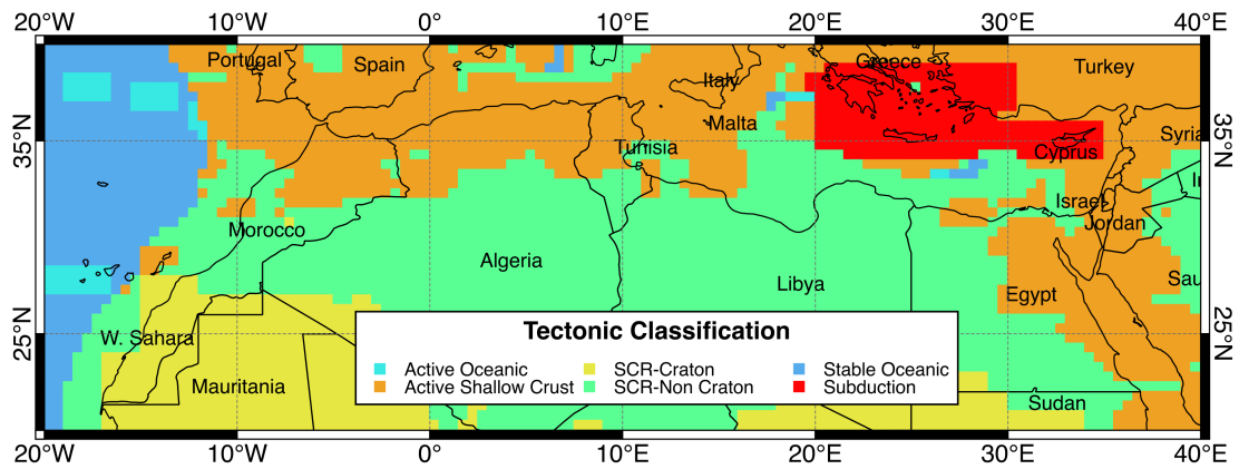
Figure 9 – Tectonic classification proposed by Chen et al. (2018) used to guide the regionalisation of the North Africa seismic source zones (see Table 10).
