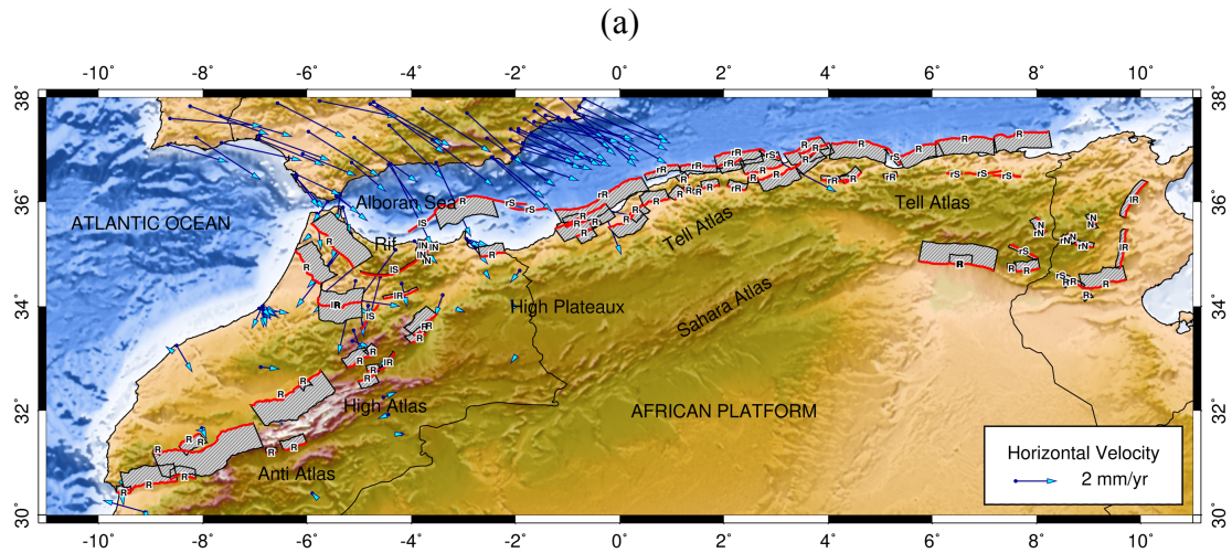
Figure 2 – Trace (in red) and surface projection (in gray) of the modelled active faults of the Maghreb (a) and Egypt (b) regions. Dominant mechanism is indicated with R (Reverse), N (Normal) or S (Strike-slip), while lateral and oblique slip components are indicated with l (left-lateral) and r (right-lateral). Measured GPS velocities are shown with blue arrows.
