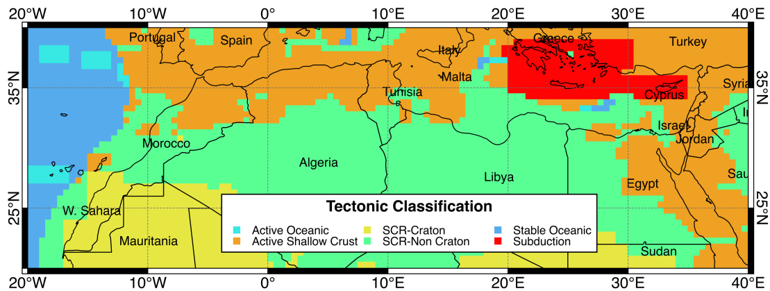
Figure 9 – Tectonic classification proposed by Chen et al. (2017) used to guide the regionalisation of the North Africa seismic source zones (see Table 9).
