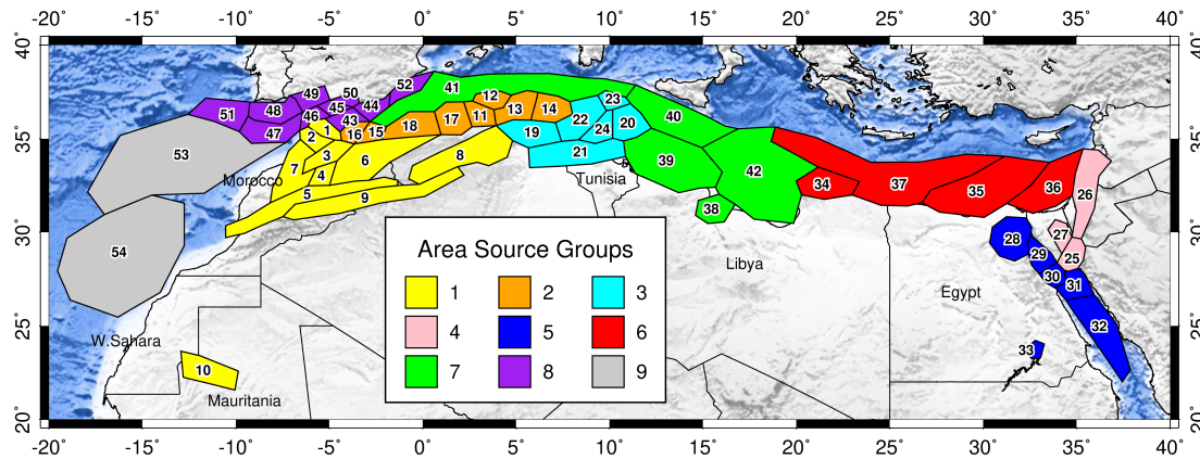
Figure 3 – The proposed source zonation for North Africa. Different colours are used to represent the 9 main tectonic groups (see Table 9) of the region.
