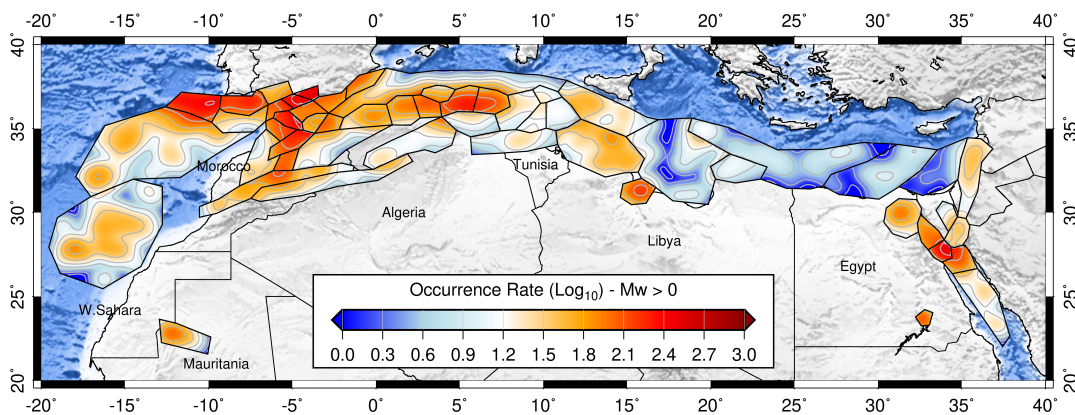
Figure 6 – Example of spatial redistribution of the cumulative annual rates ( M > 0 ) using a decay parameter ( \lambda ) of 50. Rates are intended by unit area of 0.1deg 2 (about 11km 2 ).
