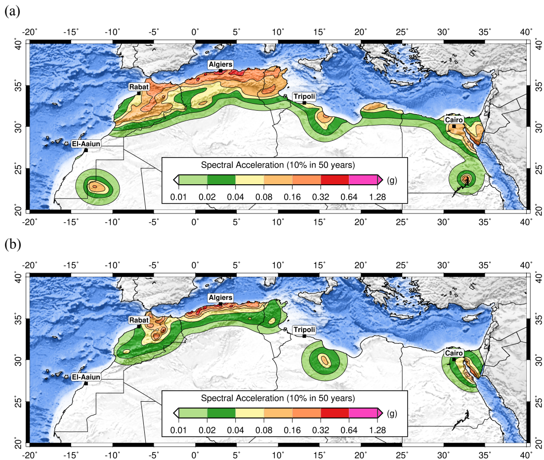
Figure 13 – Maps of spectral acceleration at PGA (g) calculated for 10% probability of exceedance in 50 years the combined source models (a) and just using the fault (b).
