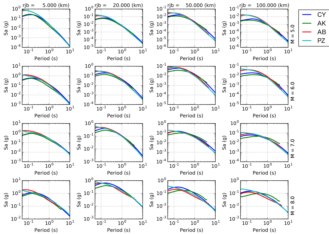
Fig. 6 Comparison between response spectra predicted by the four selected GMPEs as a function of Mw magnitude ( rows, M5 to M8) and Joyner-Boore distance (columns, 5 km to 100 km).
