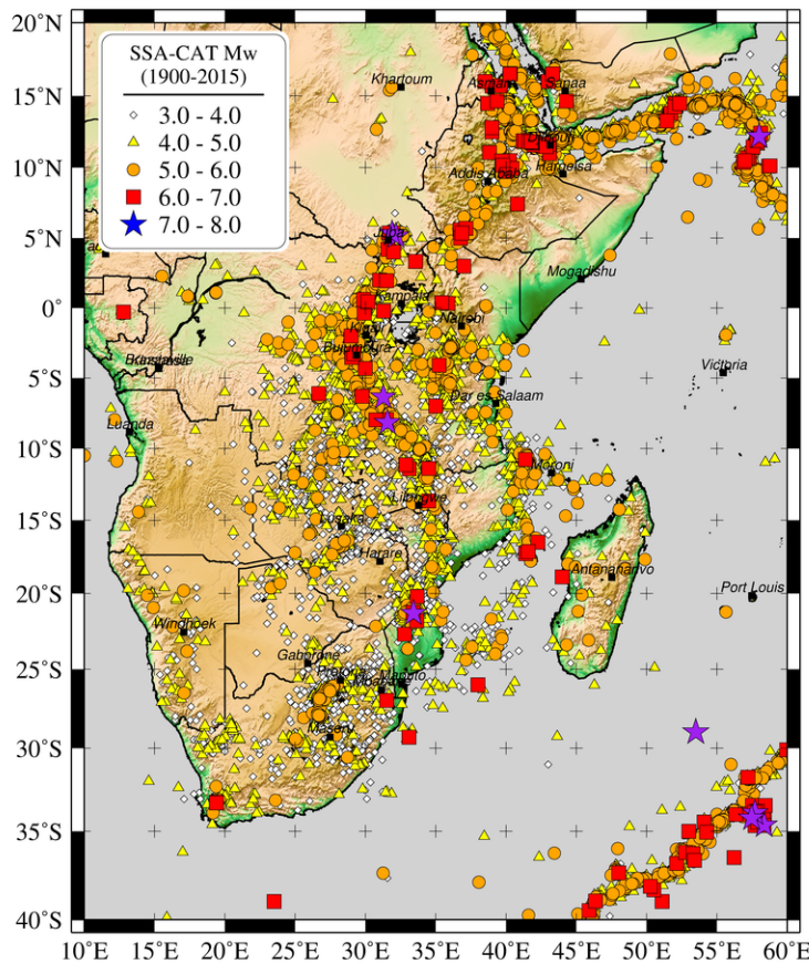
Fig. 1 Left - Distribution of events from the homogenised SSA earthquake catalogue. Bottom: Magnitude over time distribution.
