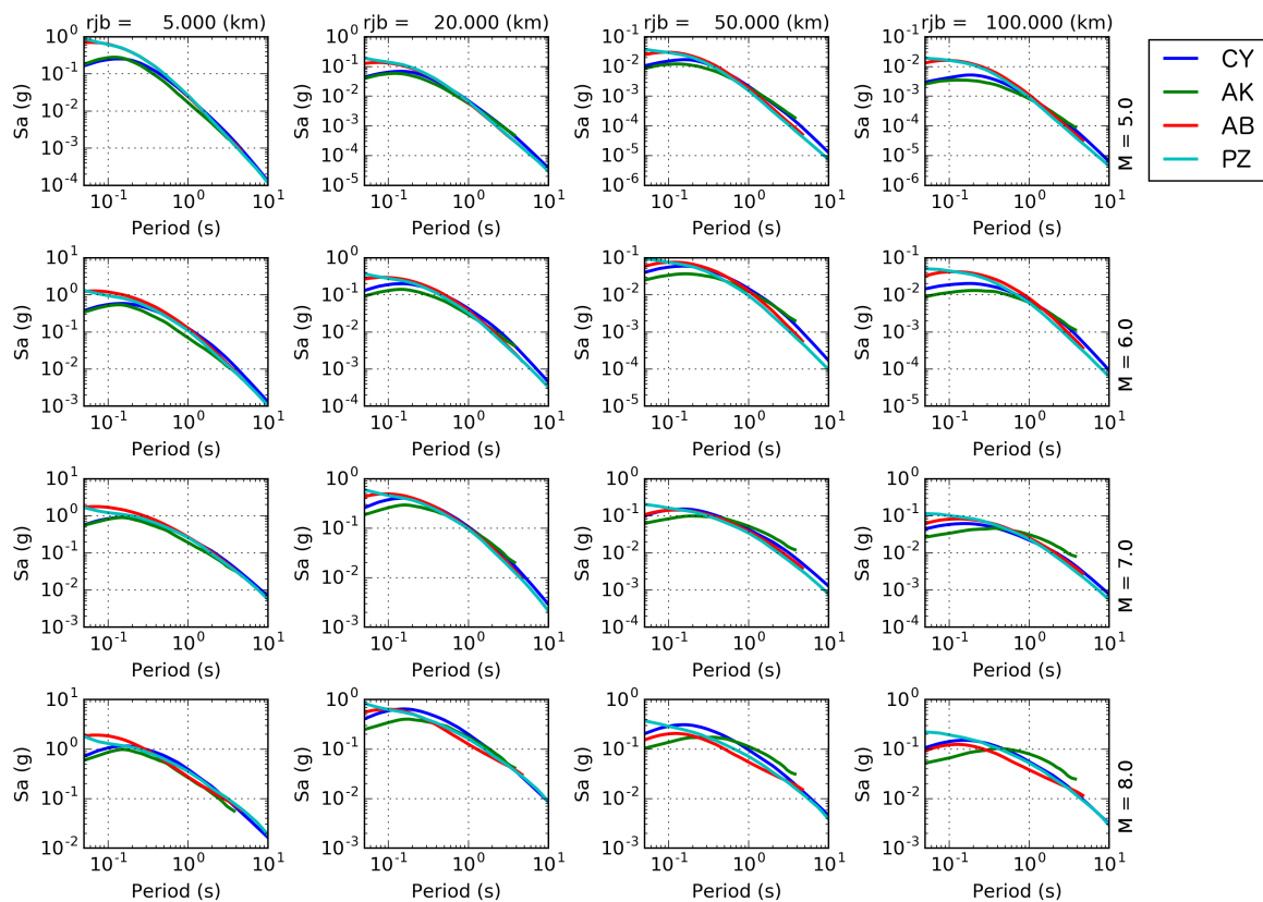
Fig. 8 Comparison between response spectra predicted by the four selected GMPEs as a function of M_w magnitude (rows, M_w 5 to M_w 8) and Joyner-Boore distance (columns, 5 km to 100 km).
