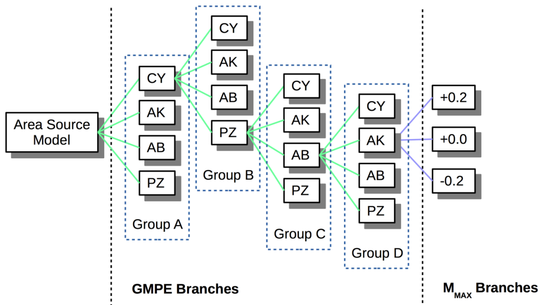
Fig. 9. Schematic representation of branch permutation for the current logic-tree implementation. Four independent branching levels are first used to characterise the four main tectonic groups (A-B-C-D) for the area. For each group, different weighting is then assigned to the selected GMPEs (see Table 5). An additional branching level is finally implemented to explore the variability of source parameters within each group. Given the explorative nature of the study, we presently only consider the uncertainty on maximum magnitude (M max ).
