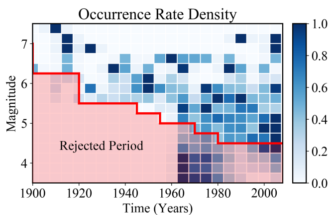
Fig. 6 Magnitude-time density plot of the SSA-GEM catalogue. Normalised rates are computed for fixed time windows of 5 years and for a 0.25 magnitude unit increment. Incomplete data periods (and other periods rejected from further interpretation) are marked with the pink shaded area.
