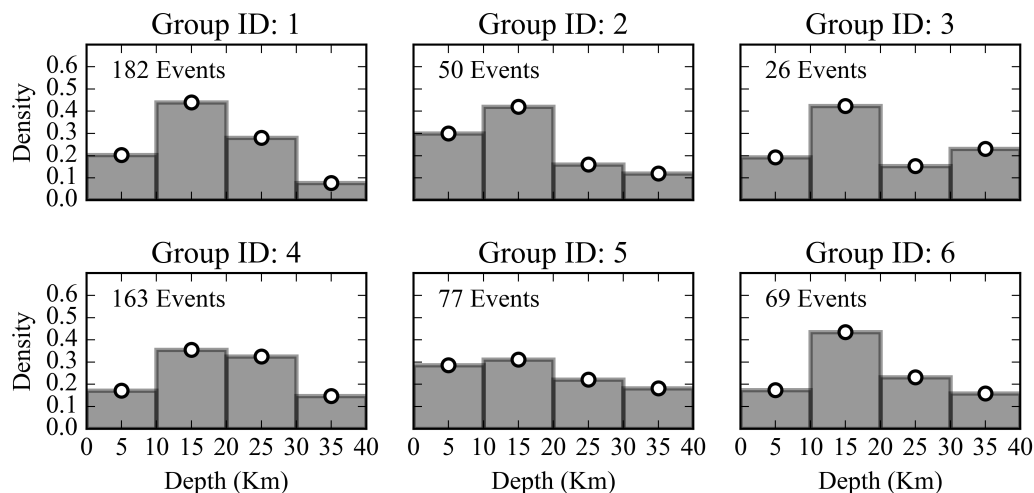
Fig. 4 Distribution of the hypocentral depth solutions of earthquake events falling into the main six source groups defined in Table 3 . The largest contribution comes persistently from the depth range between 10 km and 20 km, although many events are also observed at depths up to 40 km.
