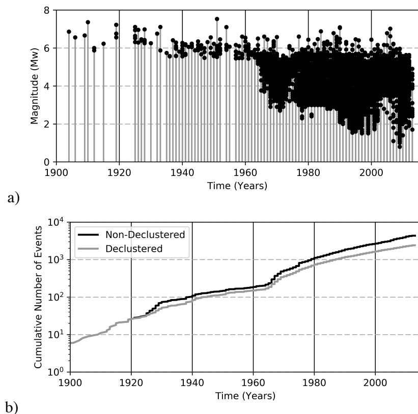
Fig. 2 a) Distribution of seismicity over time for the events in the homogenised SSA-GEM earthquake catalogue. b) Comparison between cumulative distribution of earthquakes before (non-declustered catalogue) and after fore-/aftershock cluster removal (declustered catalogue). Historical events (before 1900) are not presented.
