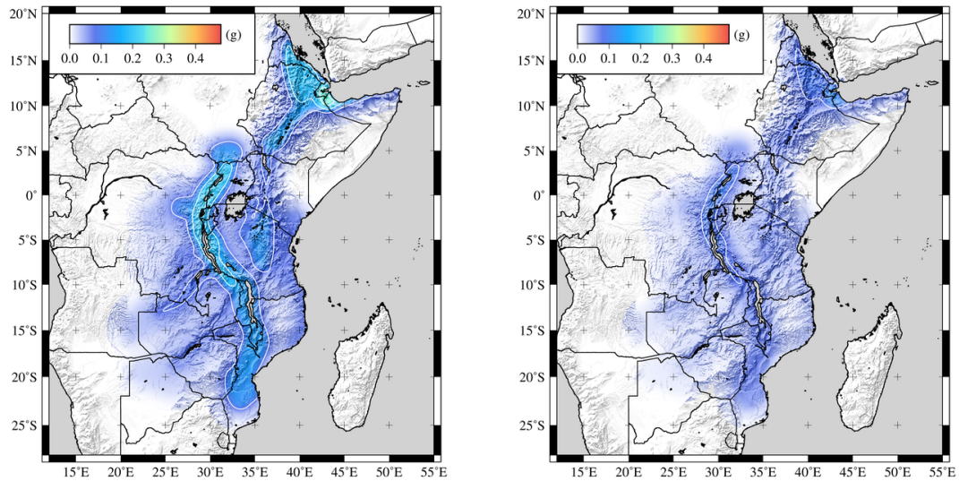
Fig. 11 Map of spectral acceleration (g) for 10% probability of exceedance in 50 years.
