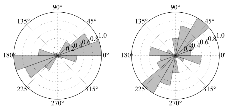
Fig. 5 Distribution of fault orientation (strike) for two example source zones (4 and 7). Input information is from the fault database of Macgregor (2015).
