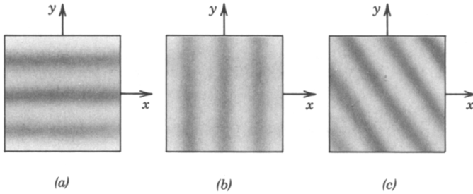
Figure A.3-1 The real part |F| \cos[2\pi\nu_x x + 2\pi\nu_y y + \arg\{F\}] of a two-dimensional harmonic function: (a) \nu_x = 0 ; (b) \nu_y = 0 ; (c) arbitrary case. For this illustration we have assumed that \arg\{F\} = 0 so that dark and white points represent positive and negative values of the function, respectively.
