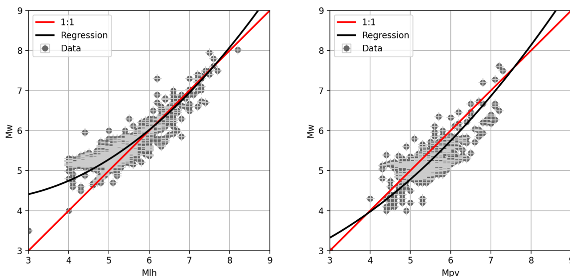
Figure 3. Magnitude conversion relations developed for Mlh and Mpv scale to Mw by fitting 2 nd degree polynomial to observed magnitude pairs using orthogonal least squares.
