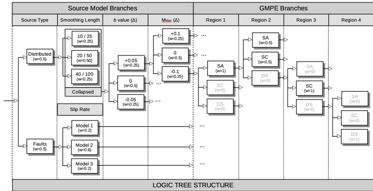
Figure 29. Diagram representation of the logic-tree structure of the Central Asia hazard model, which includes 4 branching levels for both the source model and ground motion model uncertainties.
