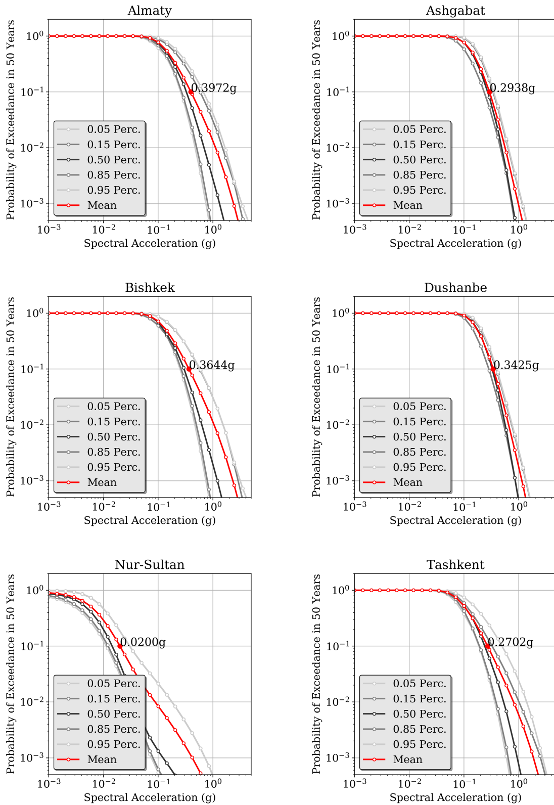
Figure 31. Example of mean hazard curve statistic (mean and quantiles) computed at six selected target sites (all country capitals plus Almaty, Kazakhstan) for PGA with 10% probability of exceedance in 50 years.
