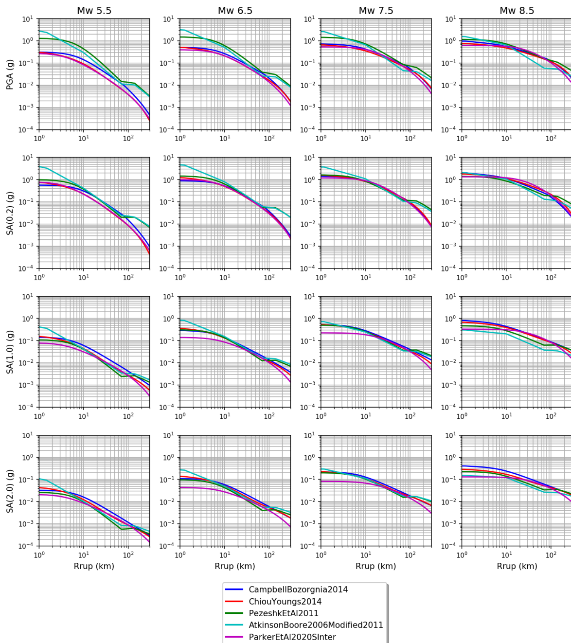
Figure 25. Comparison of ground motion distance attenuation for the view selected prediction models at different magnitudes (columns) and intensity measure types (rows).
