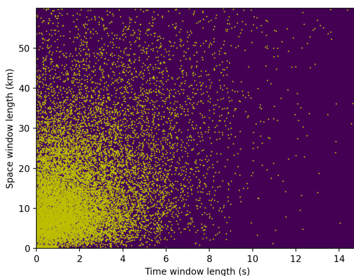
Figure 2. Time and space distance of the events identified as duplicated between the ISC bulletin and the EMCA catalogue. More than 95% of the events is captures within a 15s and 60km windows, although the bulk of events is within a 5s and 25km error.
