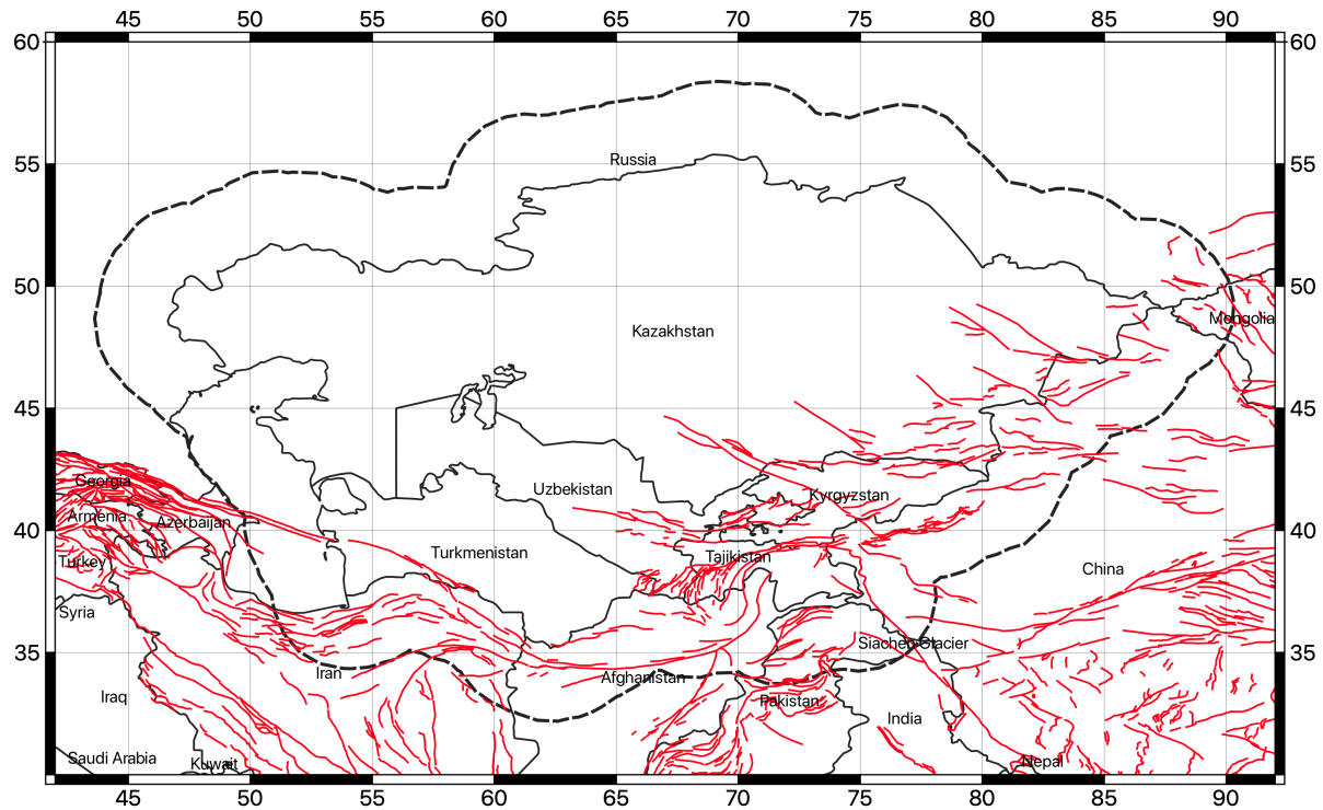
Figure 21. Faults available from the global active fault database of GEM (GEM GAF-DB).
