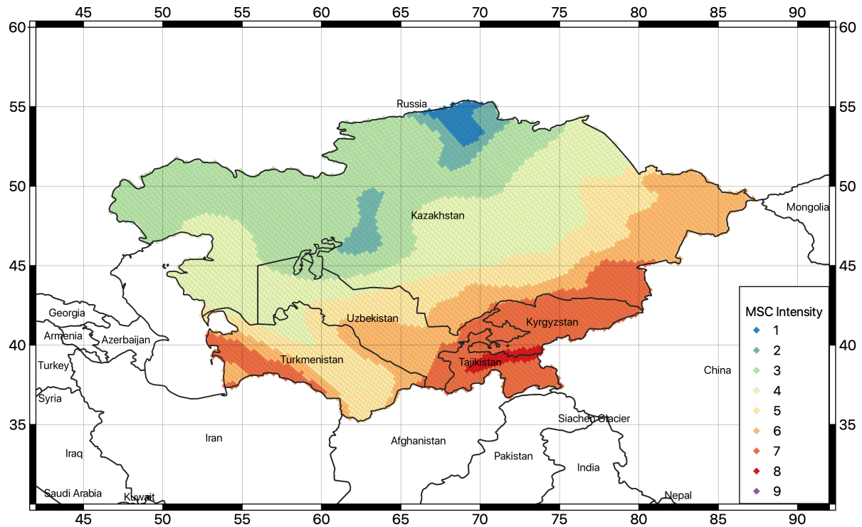
Figure 37. Map of the converted macroseismic intensity (MCS) with 63% probability of exceedance for 50 years investigation time (corresponding to about 50 years return period).
