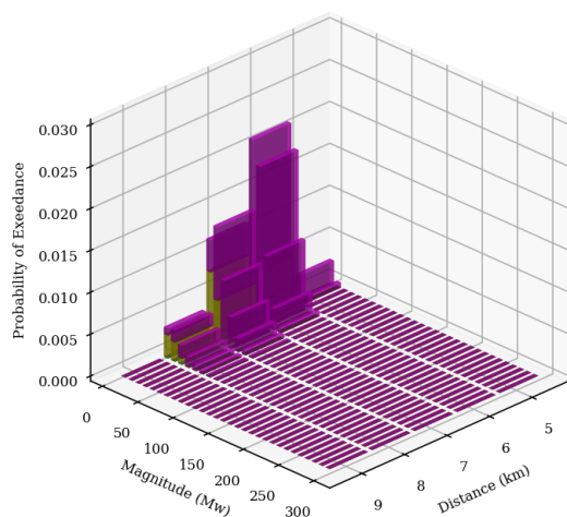
Figure 39. Magnitude-distance-epsilon disaggregation matrix computed at the six target sites for 0.2 second spectral acceleration and return period of 475 years (10% PoEs in 50 years investigation time).
