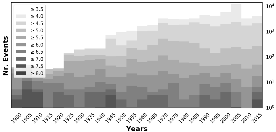
Figure 6. Number of events of the Central Asia catalog computed for five-years windows in the period 1900-2015. Shades are for bins of increasing magnitude threshold (cumulative).
