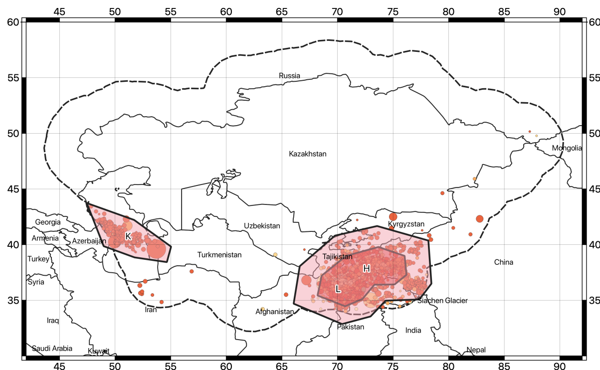
Figure 10. Earthquake source zonation model for the intermediate (50-150km) and deep (>150km) crust.
