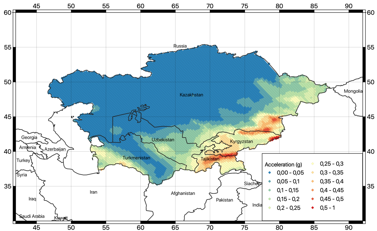
Figure 34. Map of the computed peak ground accelerations (PGA) with 10% probability of exceedance for 50 years investigation time (corresponding to about 475 years return period).
