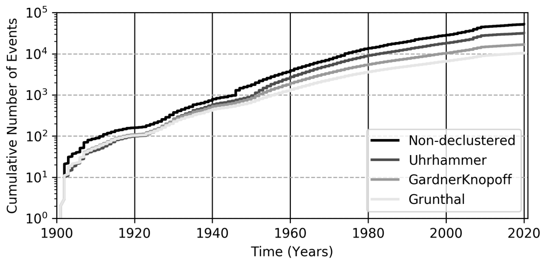
Figure 7. Cumulative number of events over time for the full (non-declustered) HECCA catalogue and when using the three tested declustering algorithms.
