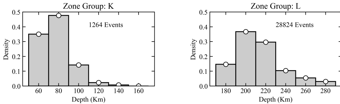
Figure 11. Probability density distribution of the earthquake hypocentral depths for the main tectonic groups of the Central Asia source model (A-G shallow depth sources, H-K intermediate depth sources, L deep sources).
