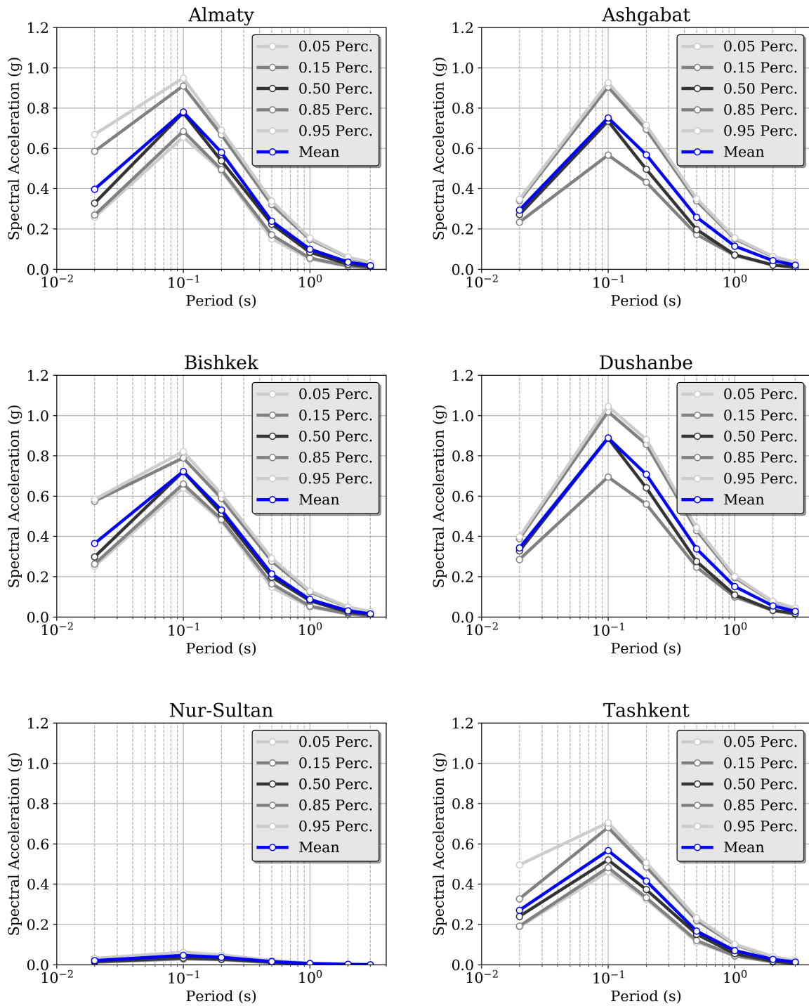
Figure 32. Example of uniform hazard spectra (UHS) computed at six selected target sites (all country capitals plus Almaty, Kazakhstan) for 10% probability of exceedance in 50 years.
