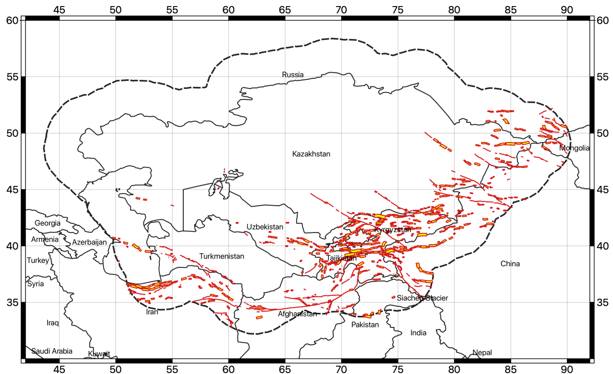
Figure 22. 3D geometry of the faults in the final source model. Surface traces are in red, while the surface projection of the fault plane is in yellow.
