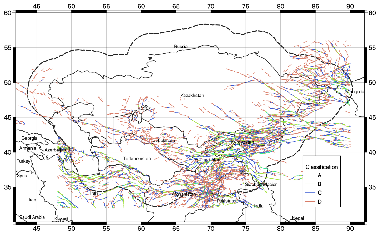
Figure 20. Faults available from the database of Active Fault for Eurasia and adjacent regions (AFEAD)
