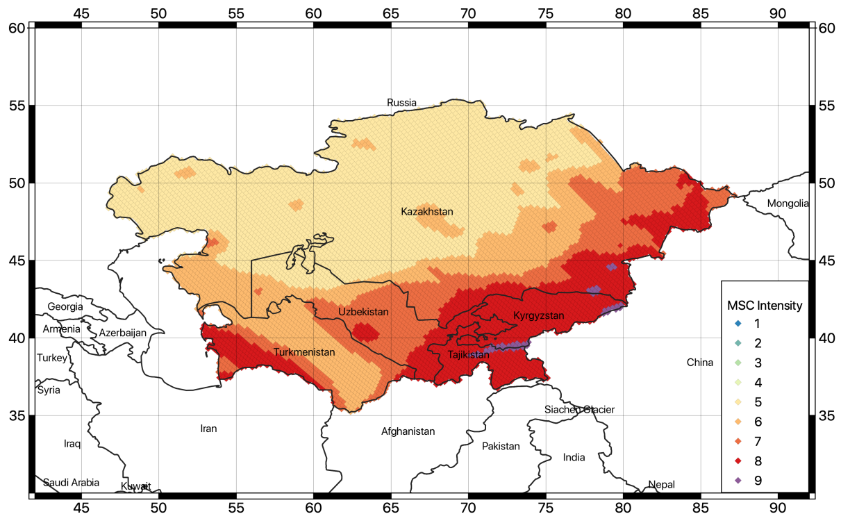
Figure 38. Map of the converted macroseismic intensity (MCS) with 10% probability of exceedance for 50 years investigation time (corresponding to about 475 years return period).
